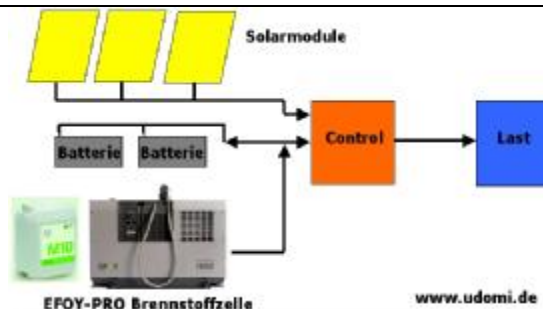
EFOY-PRO – PV Hybride System
