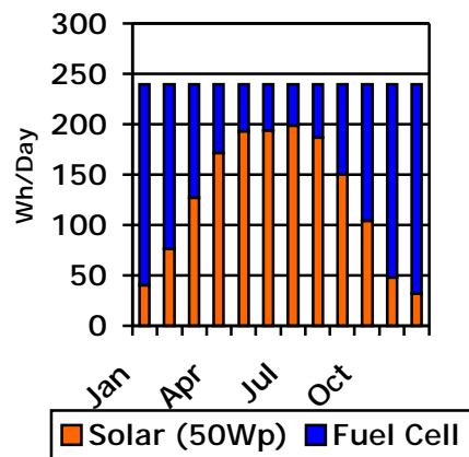
EFOY-OUTDOOR hybrid solution example for 10 Watt continuous power (240Wh/day)
